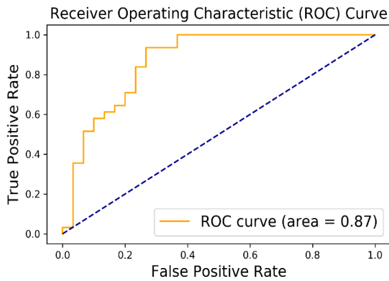
Fig 4: ROC curve showing the performance output of Gaussian Naïve Bayes model
